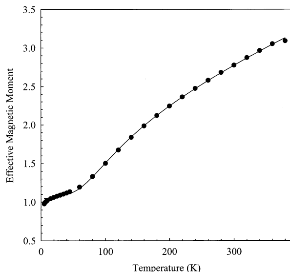
Figure 3. Plot of effective magnetic moment versus temperature for [\text{Fe}_2(\text{O})(\text{O}_2\text{CCH}_2\text{C}_{10}\text{H}_7)_2(\text{TACN-Me}_3)_2](\text{PF}_6)_2 ( 3 , ●) in the solid state. The solid line represents the theoretical fit of the data. See text for further details.
