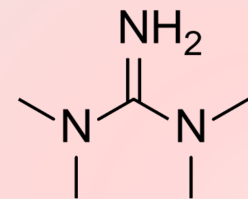
Tetramethylguanidine
