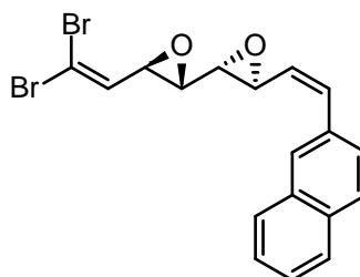
enantiomer shown Problem 195 G
