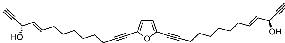
enantiomer shown Problem 109 G
