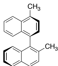
enantiomer shown Problem 136
