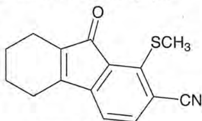
Molecule A
