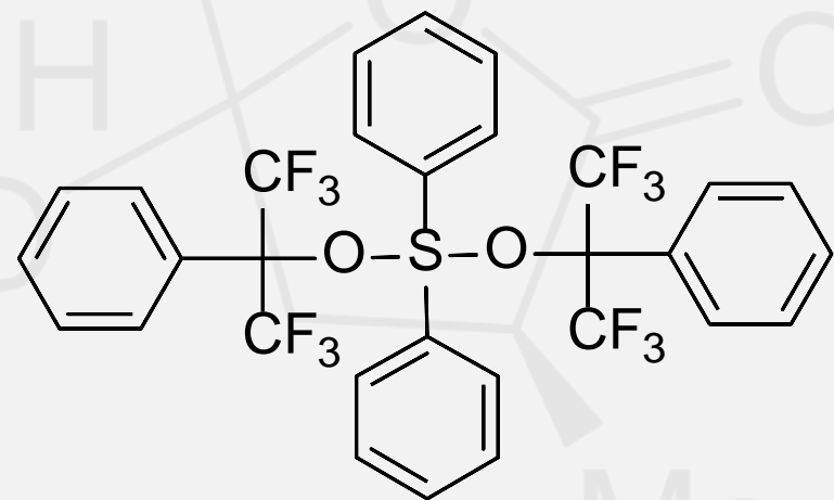
Martin's Sulfurane
