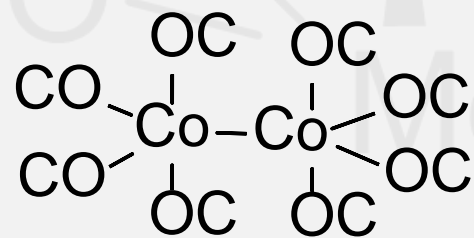
Dicobalt Octacarbonyl
