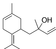
humbertiol
