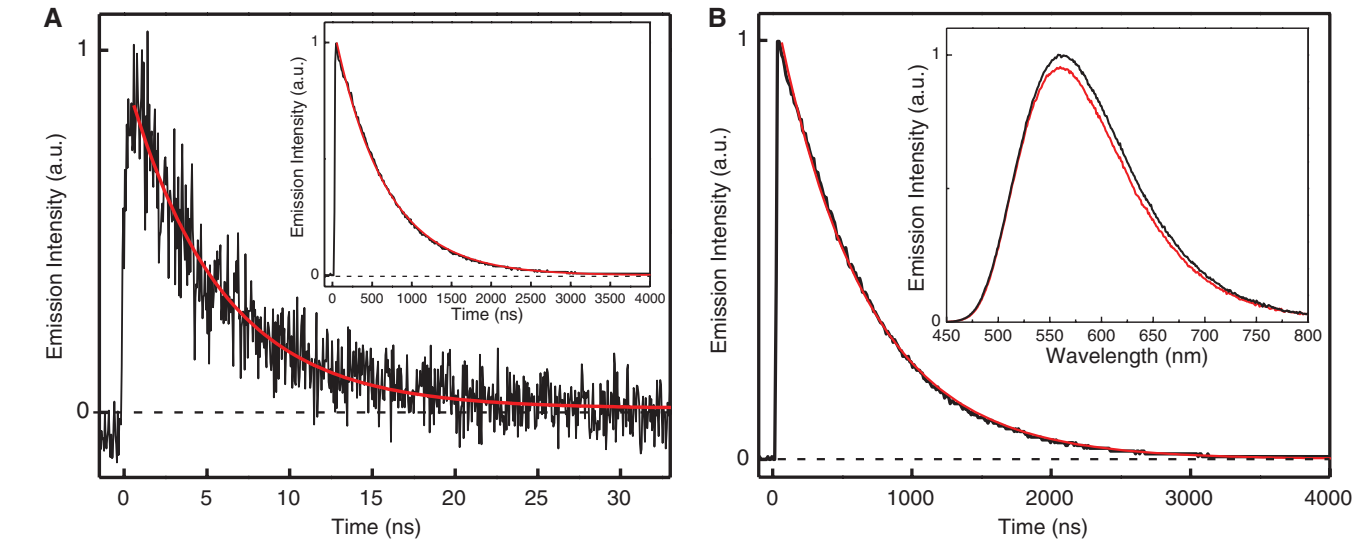
Fig. 3. (A) Time-correlated single-photon counting data for CrRe 3 (1) at λ = 580 nm after excitation at 375 nm, fit to a single-exponential decay model (red line) with τ obs = 4.8 ± 0.2 ns. Inset: Nanosecond time-resolved emission data for GaRe 3 (3) at λ = 580 nm after excitation at 400 nm, fit to a single-exponential decay model (red line) with τ obs = 630 ± 30 ns. All data were collected at room temperature in deoxygenated CH 2 Cl 2 solutions. (B) Nano-
